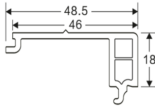
SHUTTER GLAZING BEAD WITH HOLE LENGTH (5.9 MTR ) 0.260 KG/M
